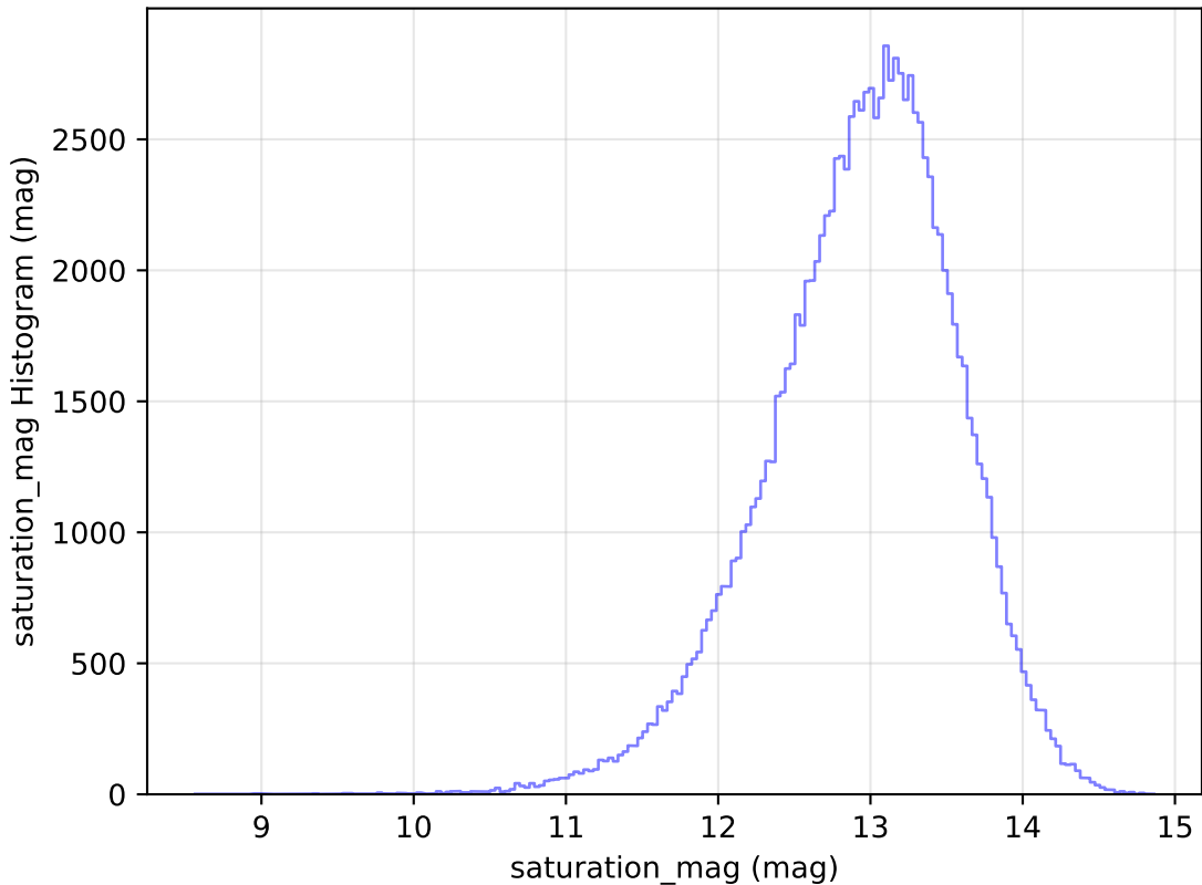
extra_ss_neo7_v3.4_10yrs All sky u band: saturation_mag Histogram
