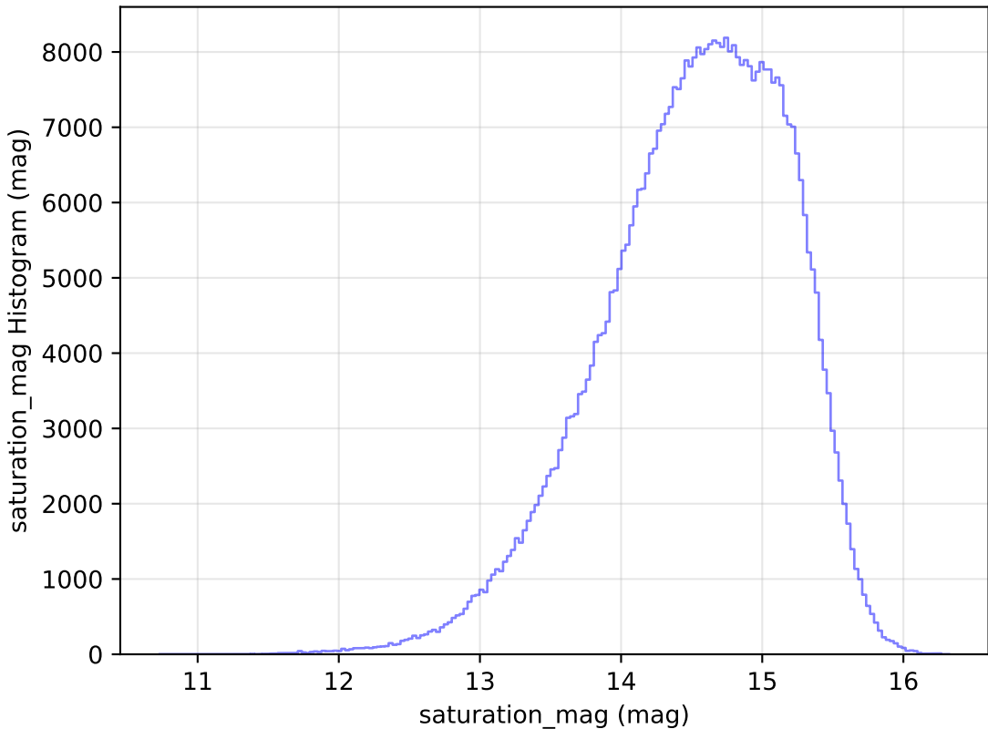
extra_ss_neo7_v3.4_10yrs All sky r band: saturation_mag Histogram
