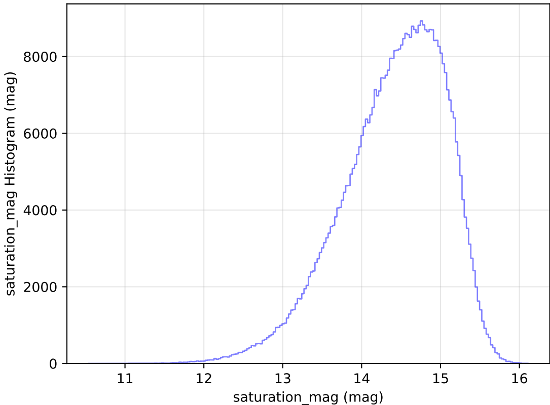
extra_ss_neo7_v3.4_10yrs All sky i band: saturation_mag Histogram
