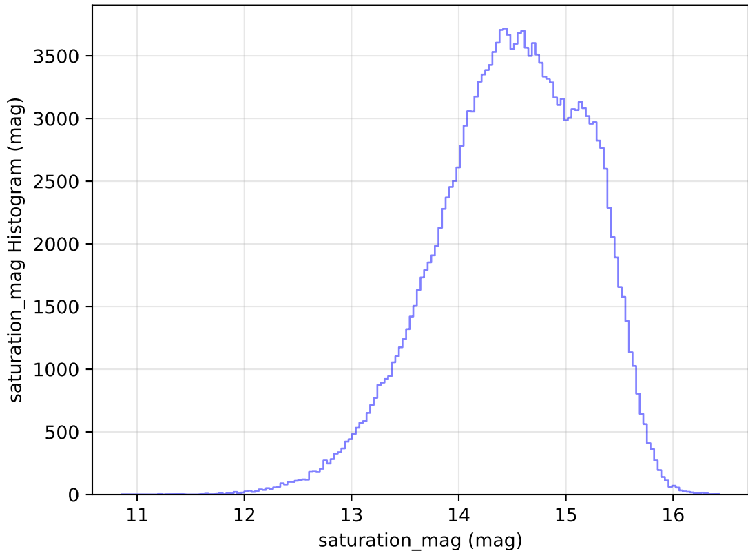
extra_ss_neo7_v3.4_10yrs All sky g band: saturation_mag Histogram
