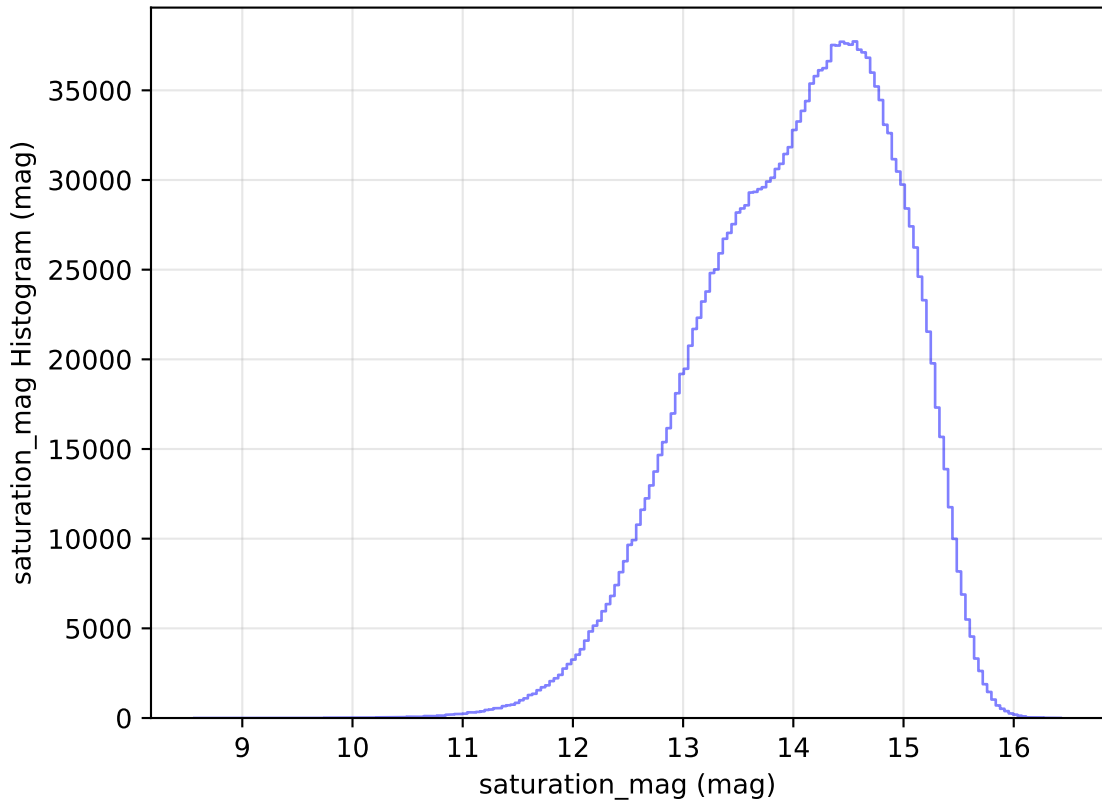
extra_ss_neo7_v3.4_10yrs All sky all bands: saturation_mag Histogram
