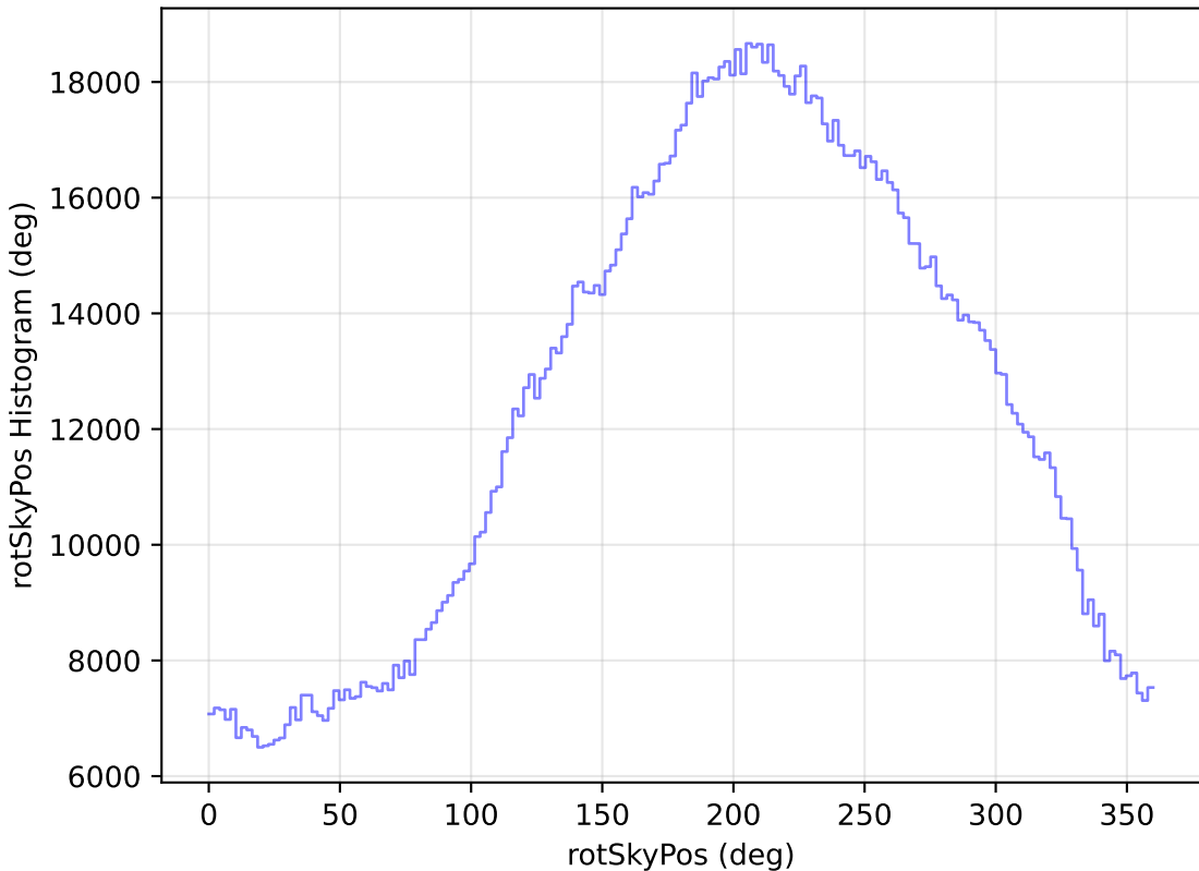
extra_ss_neo7_v3.4_10yrs All sky all bands: rotSkyPos Histogram
