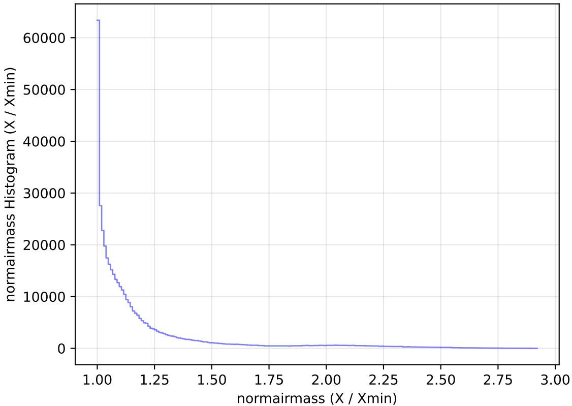
extra_ss_neo7_v3.4_10yrs WFD z band: normairmass Histogram
