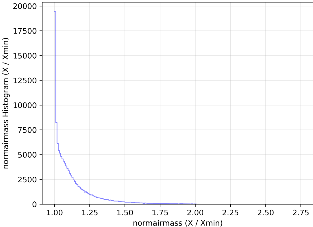
extra_ss_neo7_v3.4_10yrs WFD u band: normairmass Histogram
