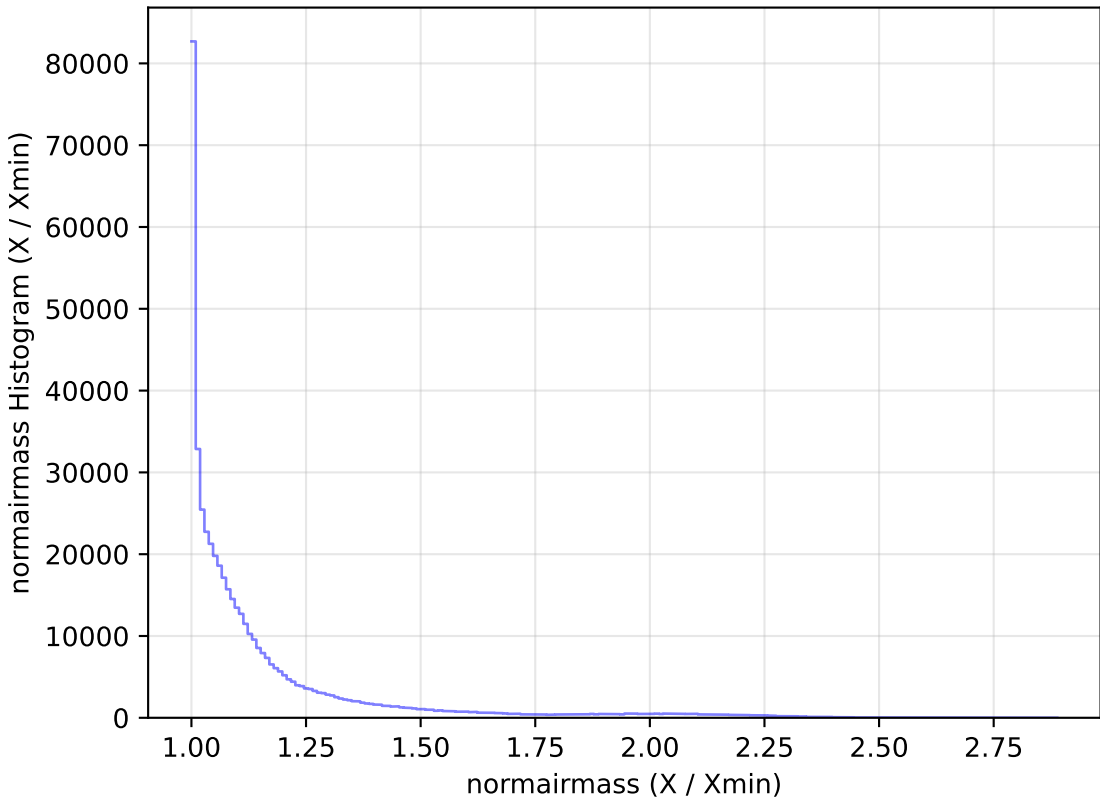
extra_ss_neo7_v3.4_10yrs WFD r band: normairmass Histogram
