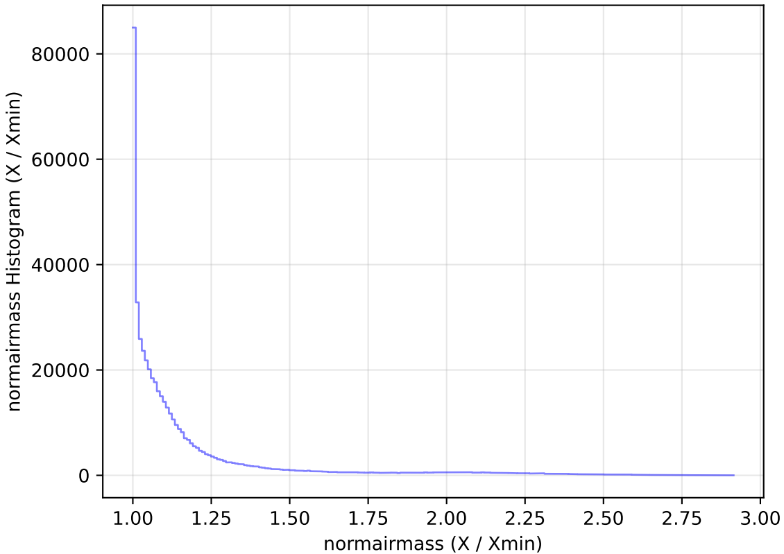
extra_ss_neo7_v3.4_10yrs WFD i band: normairmass Histogram
