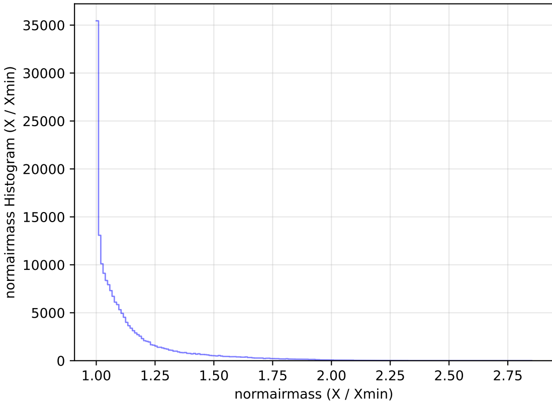
extra_ss_neo7_v3.4_10yrs WFD g band: normairmass Histogram
