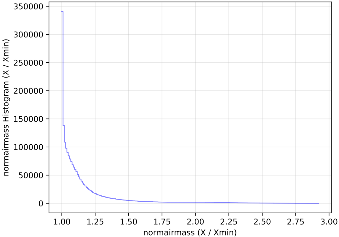
extra_ss_neo7_v3.4_10yrs WFD all bands: normairmass Histogram
