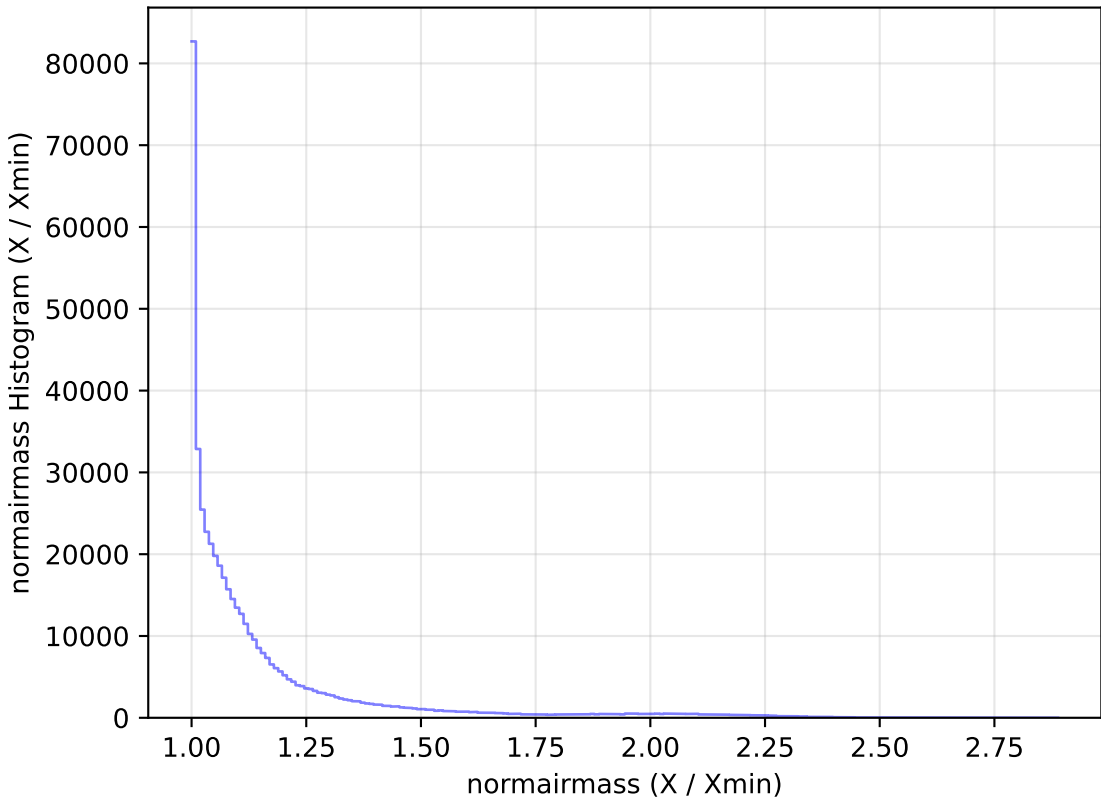
extra_ss_neo7_v3.4_10yrs All sky r band: normairmass Histogram
