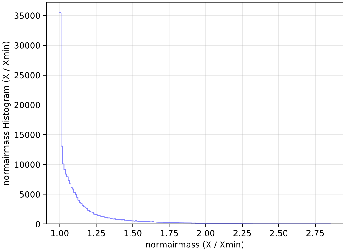
extra_ss_neo7_v3.4_10yrs All sky g band: normairmass Histogram
