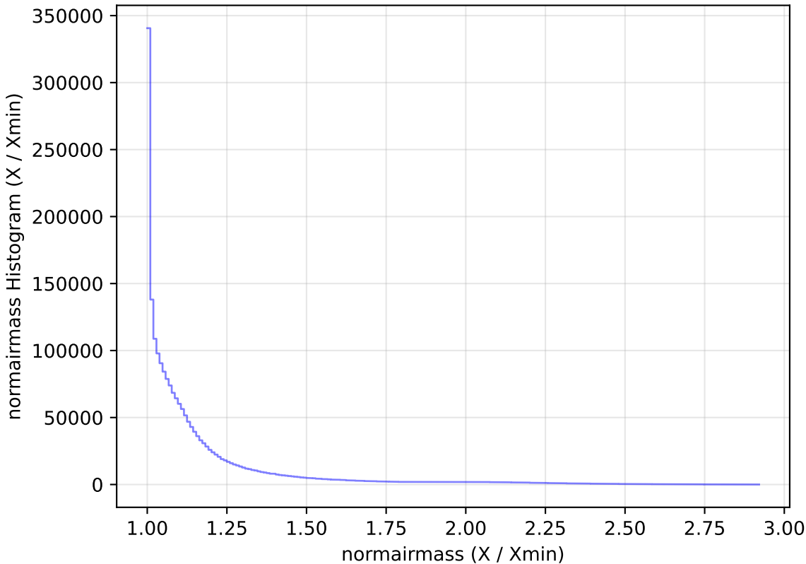
extra_ss_neo7_v3.4_10yrs All sky all bands: normairmass Histogram
