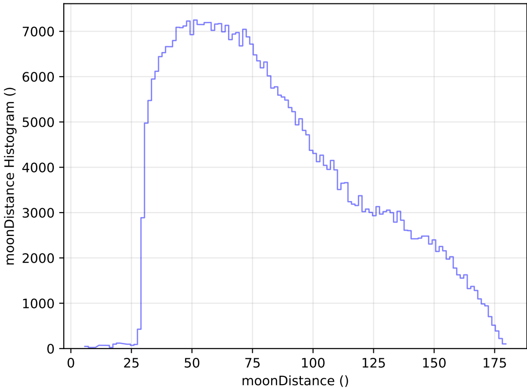
extra_ss_neo7_v3.4_10yrs WFD z band: moonDistance Histogram
