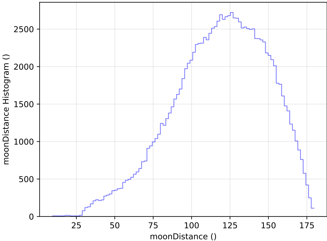
extra_ss_neo7_v3.4_10yrs WFD u band: moonDistance Histogram
