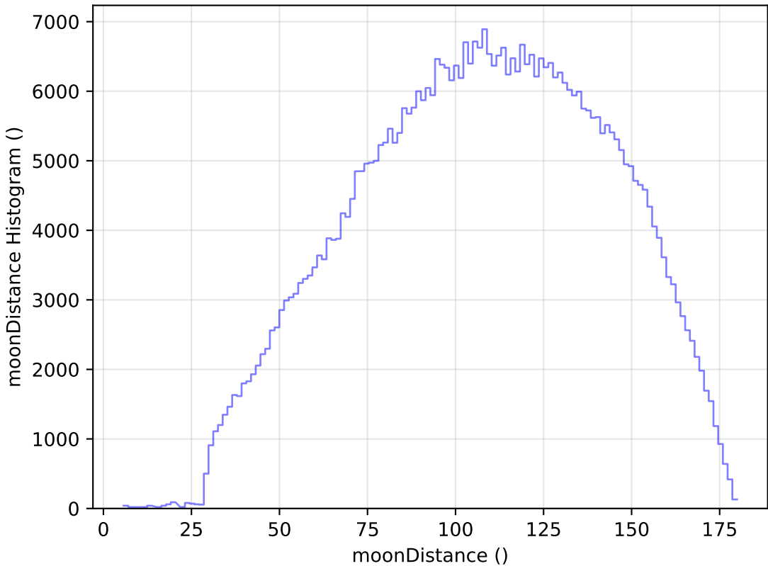
extra_ss_neo7_v3.4_10yrs WFD r band: moonDistance Histogram
