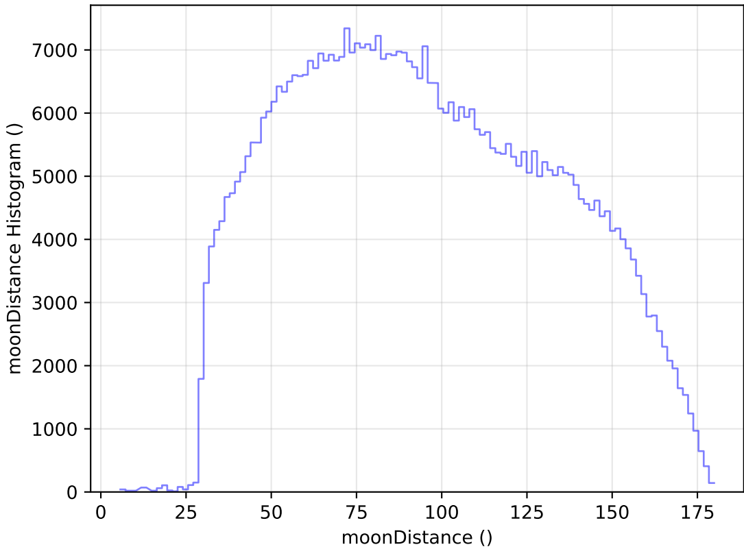
extra_ss_neo7_v3.4_10yrs WFD i band: moonDistance Histogram
