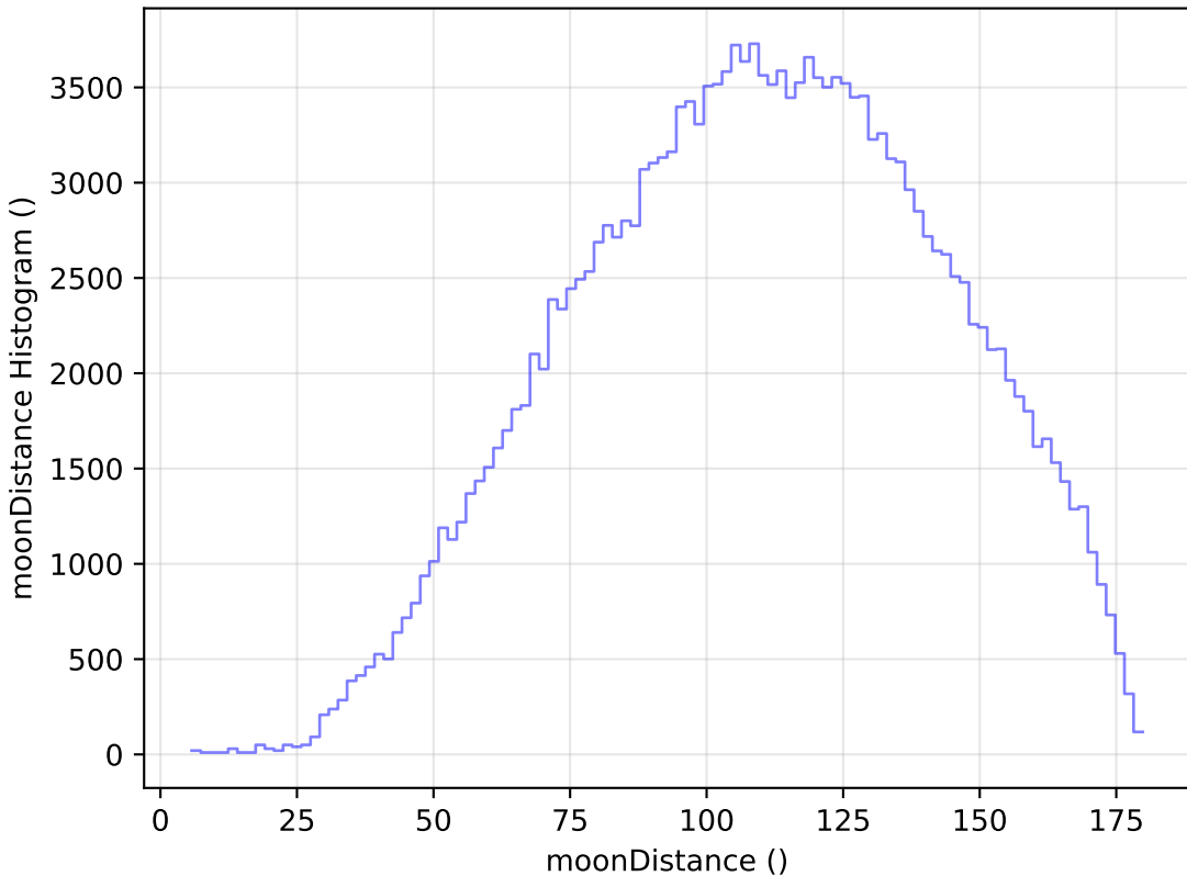
extra_ss_neo7_v3.4_10yrs WFD g band: moonDistance Histogram
