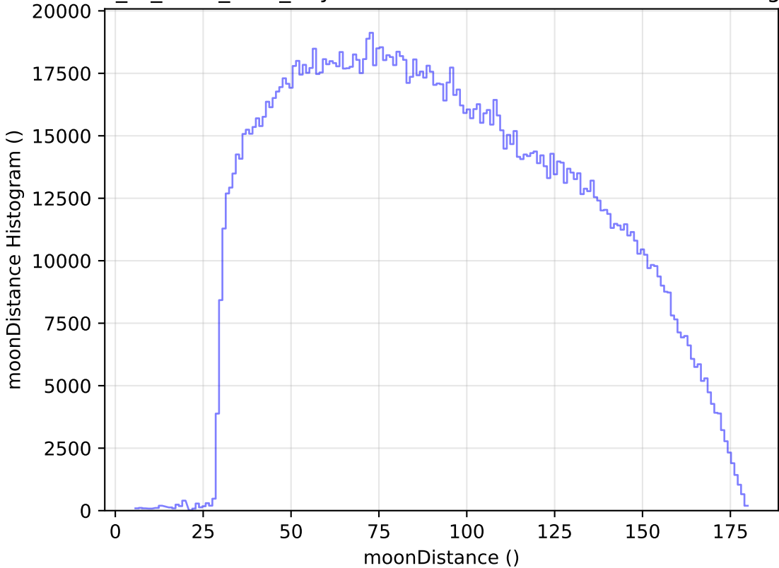
extra_ss_neo7_v3.4_10yrs WFD all bands: moonDistance Histogram
