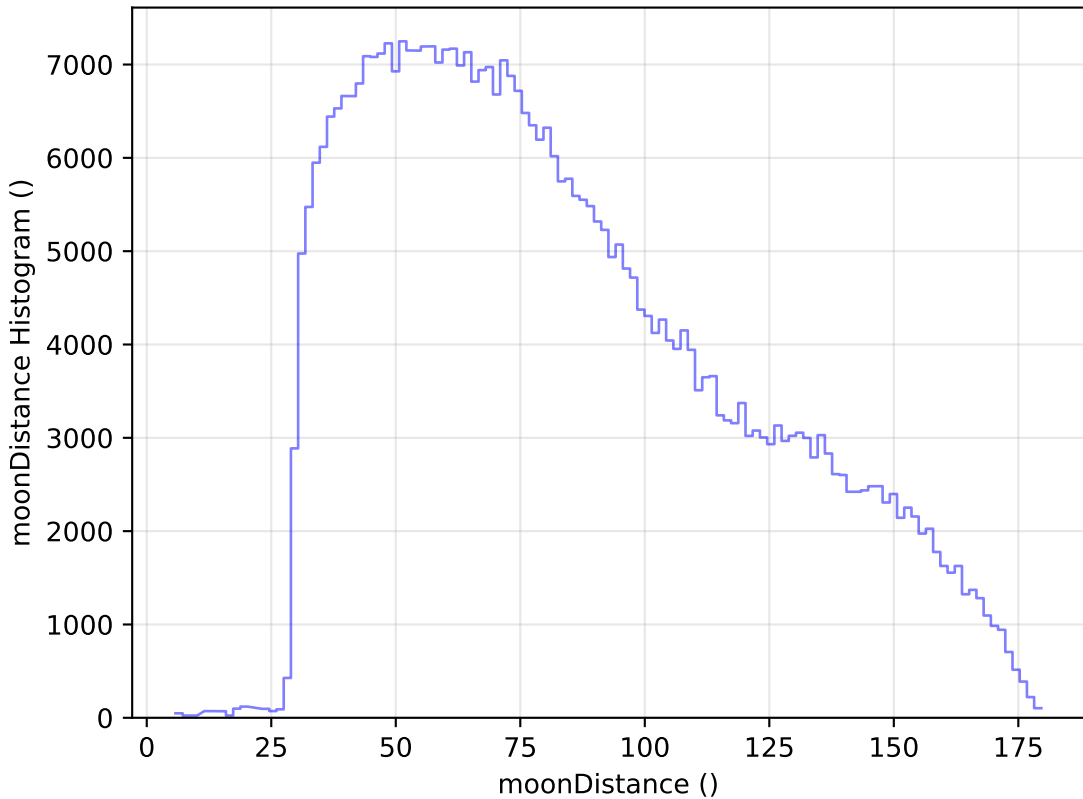
extra_ss_neo7_v3.4_10yrs All sky z band: moonDistance Histogram
