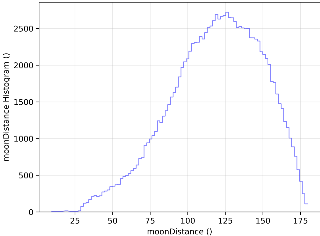
extra_ss_neo7_v3.4_10yrs All sky u band: moonDistance Histogram
