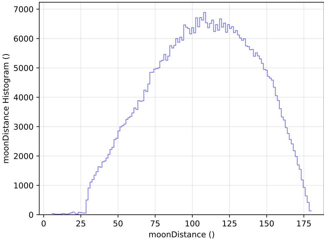
extra_ss_neo7_v3.4_10yrs All sky r band: moonDistance Histogram
