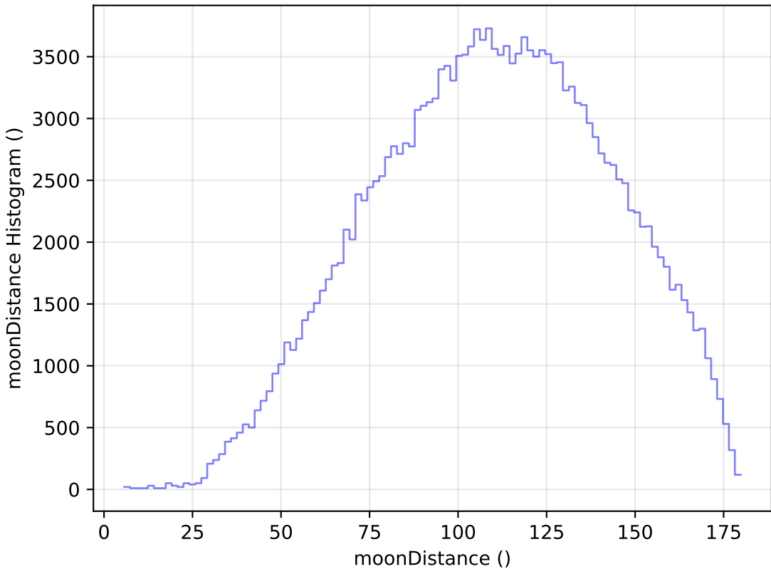
extra_ss_neo7_v3.4_10yrs All sky g band: moonDistance Histogram
