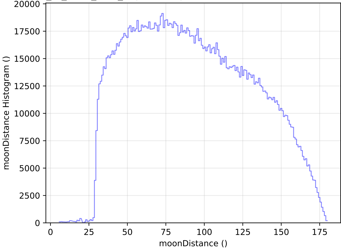
extra_ss_neo7_v3.4_10yrs All sky all bands: moonDistance Histogram
