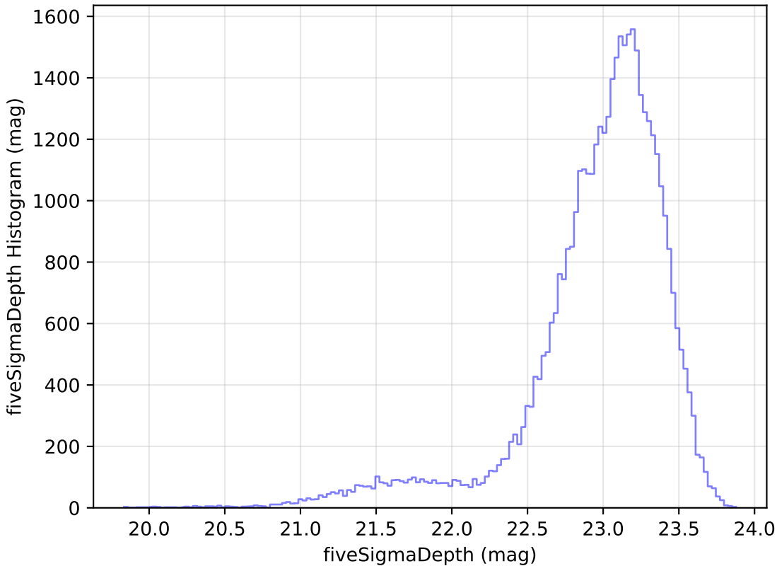
extra_ss_neo7_v3.4_10yrs Yr 1 z band: fiveSigmaDepth Histogram
