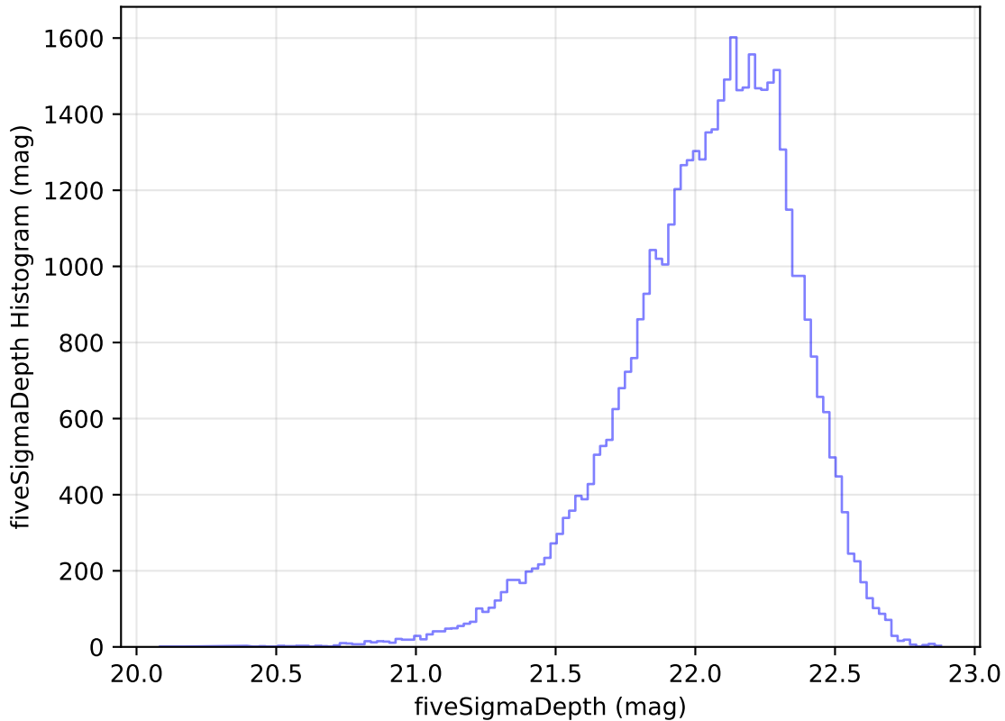
extra_ss_neo7_v3.4_10yrs Yr 1 y band: fiveSigmaDepth Histogram
