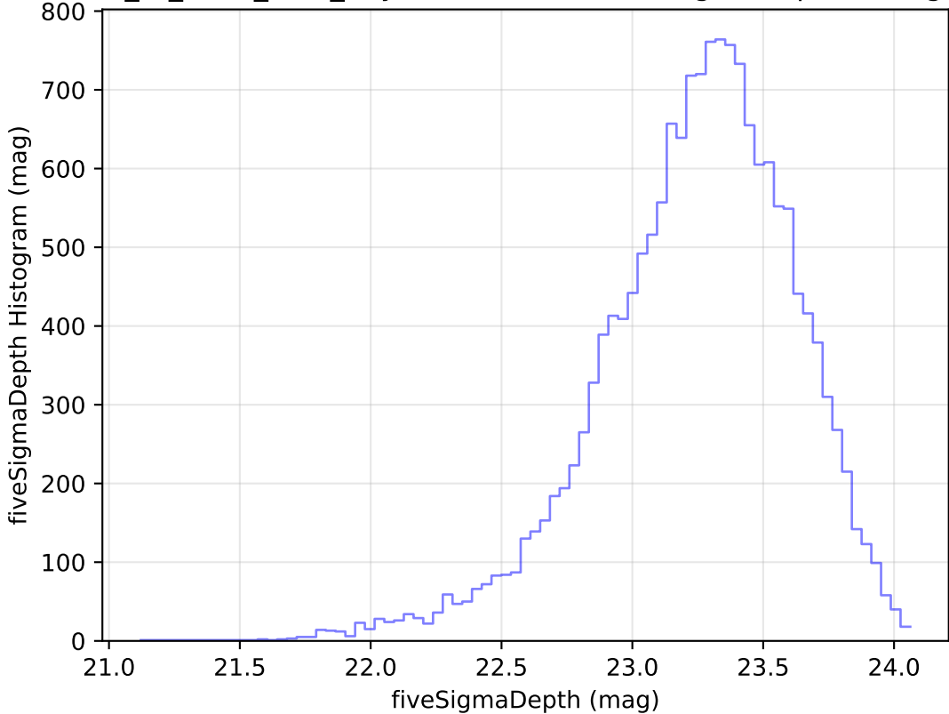
extra_ss_neo7_v3.4_10yrs Yr 1 u band: fiveSigmaDepth Histogram
