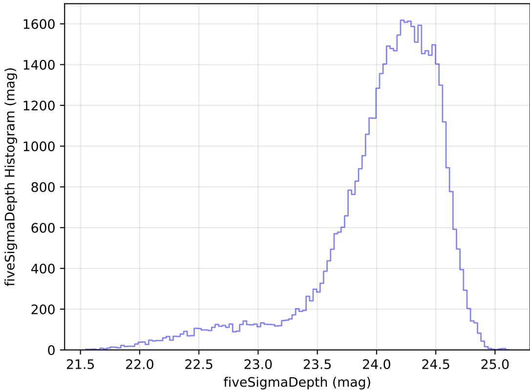
extra_ss_neo7_v3.4_10yrs Yr 1 r band: fiveSigmaDepth Histogram
