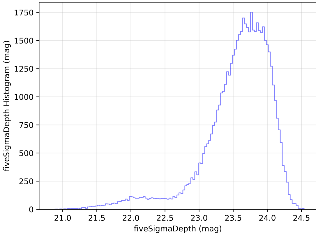
extra_ss_neo7_v3.4_10yrs Yr 1 i band: fiveSigmaDepth Histogram
