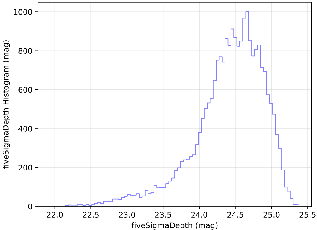
extra_ss_neo7_v3.4_10yrs Yr 1 g band: fiveSigmaDepth Histogram
