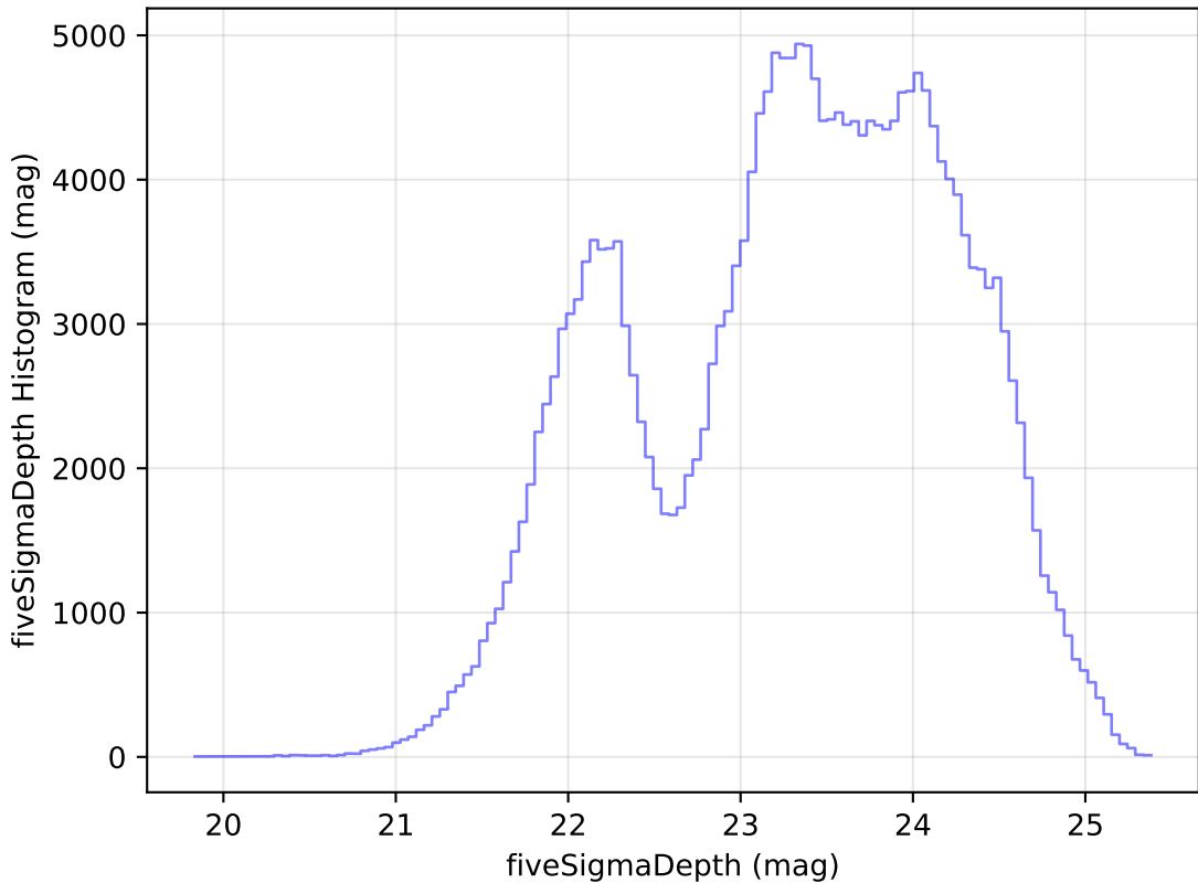
extra_ss_neo7_v3.4_10yrs Yr 1 all bands: fiveSigmaDepth Histogram
