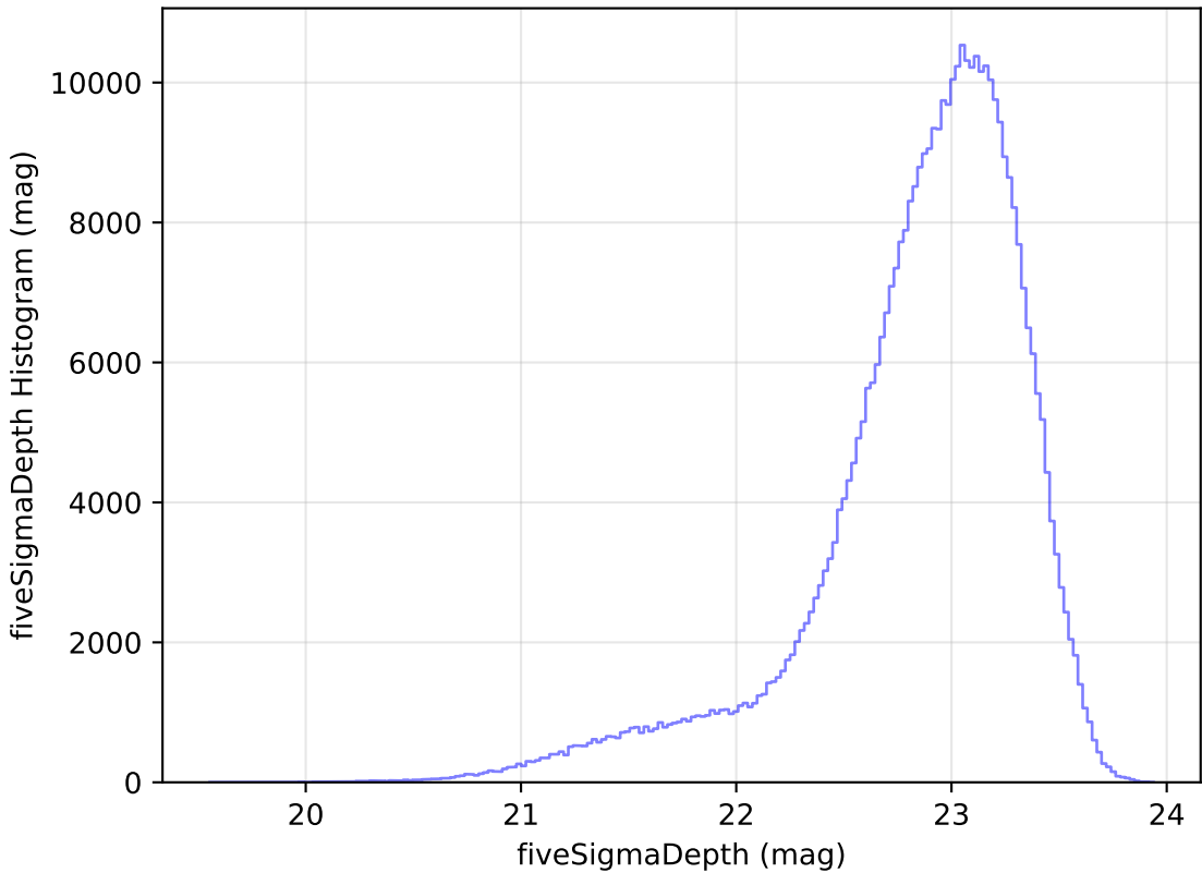
extra_ss_neo7_v3.4_10yrs WFD z band: fiveSigmaDepth Histogram
