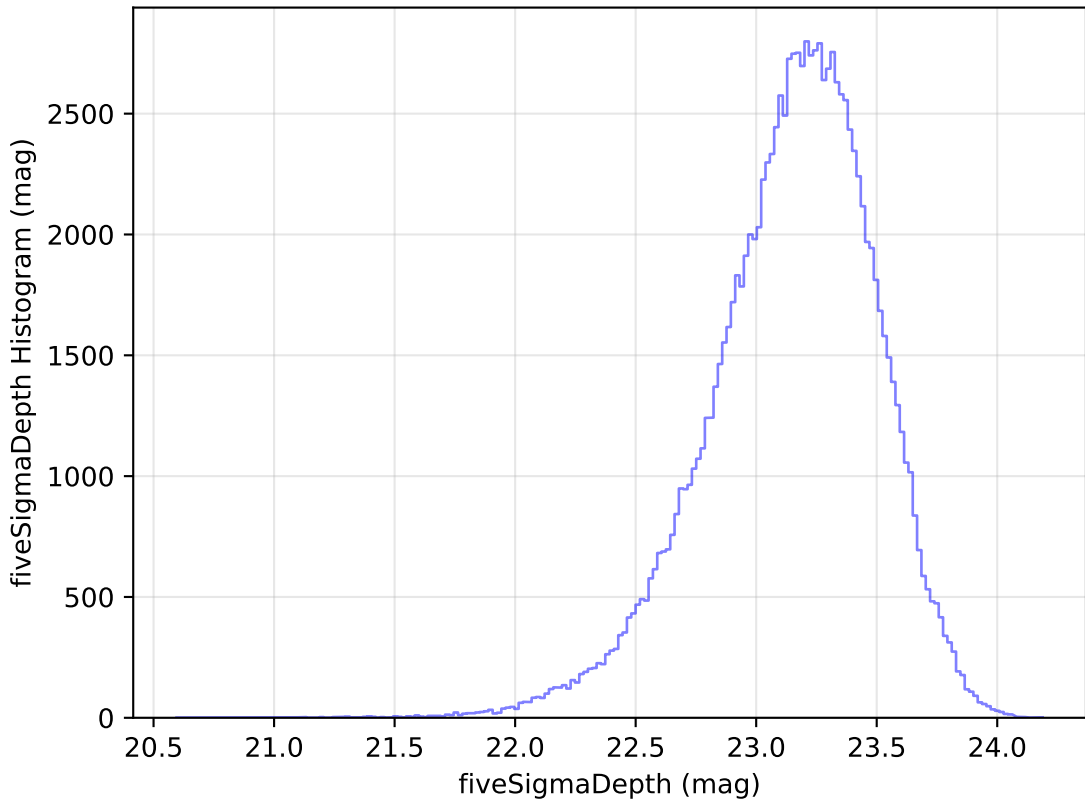
extra_ss_neo7_v3.4_10yrs WFD u band: fiveSigmaDepth Histogram
