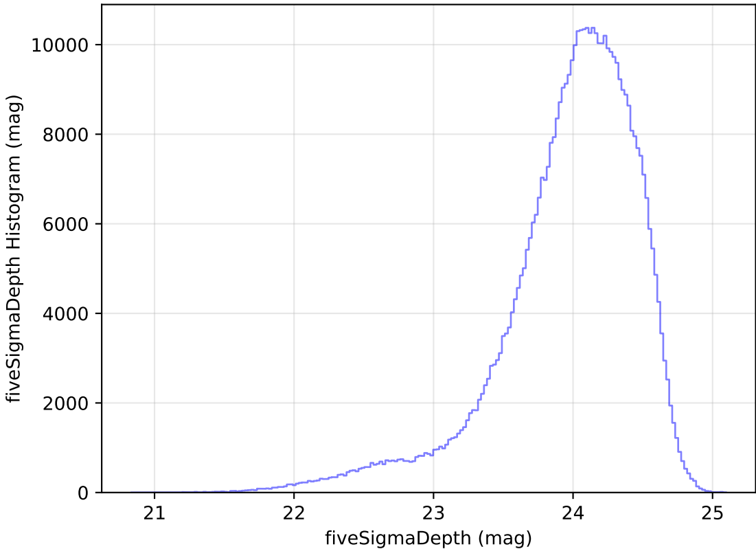
extra_ss_neo7_v3.4_10yrs WFD r band: fiveSigmaDepth Histogram
