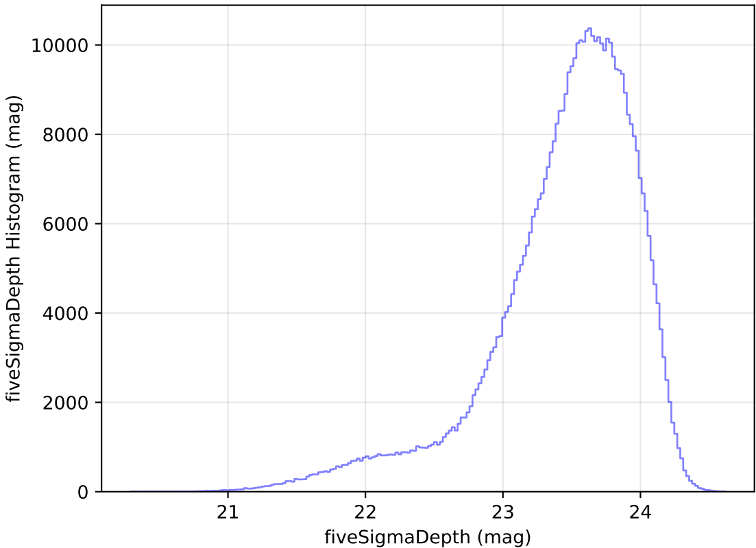
extra_ss_neo7_v3.4_10yrs WFD i band: fiveSigmaDepth Histogram
