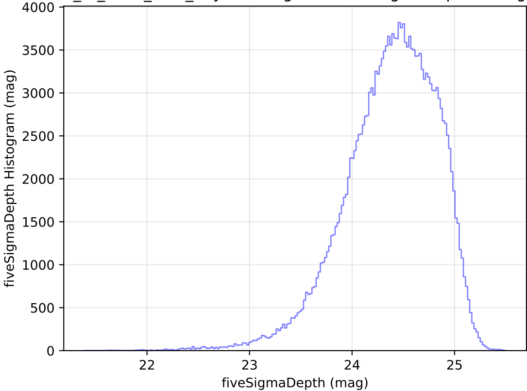
extra_ss_neo7_v3.4_10yrs WFD g band: fiveSigmaDepth Histogram
