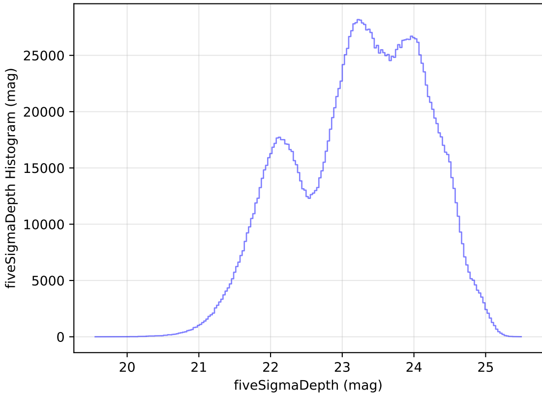
extra_ss_neo7_v3.4_10yrs WFD all bands: fiveSigmaDepth Histogram
