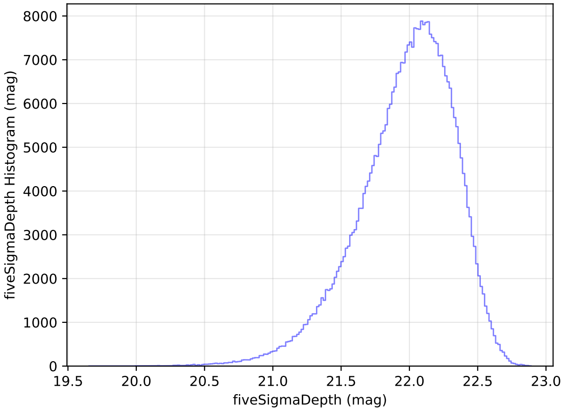
extra_ss_neo7_v3.4_10yrs All sky y band: fiveSigmaDepth Histogram
