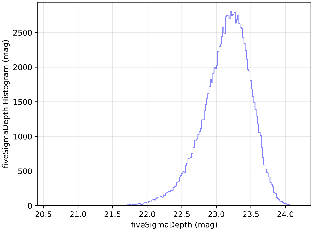
extra_ss_neo7_v3.4_10yrs All sky u band: fiveSigmaDepth Histogram
