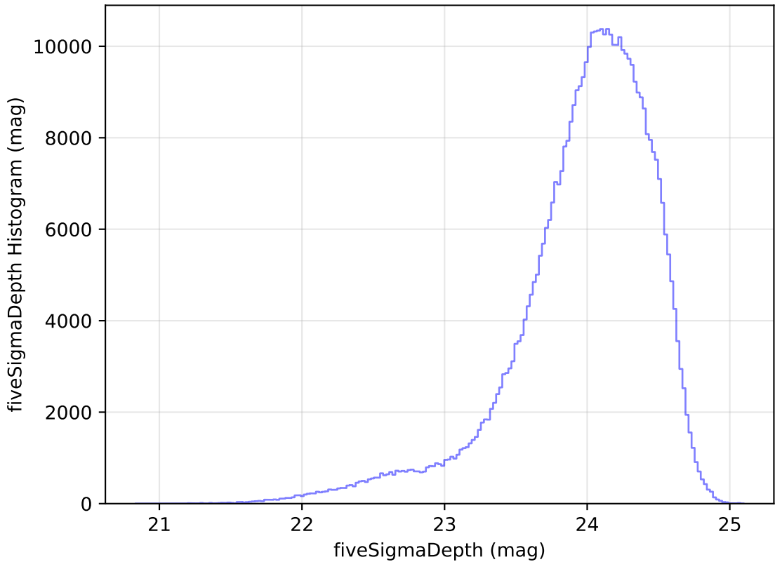
extra_ss_neo7_v3.4_10yrs All sky r band: fiveSigmaDepth Histogram
