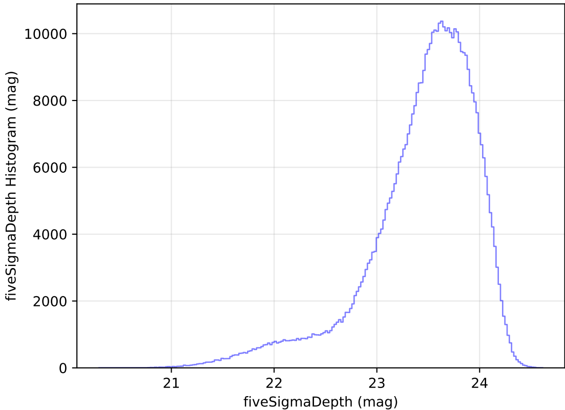
extra_ss_neo7_v3.4_10yrs All sky i band: fiveSigmaDepth Histogram
