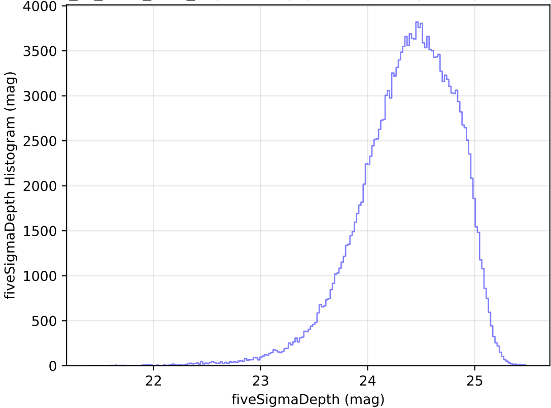
extra_ss_neo7_v3.4_10yrs All sky g band: fiveSigmaDepth Histogram
