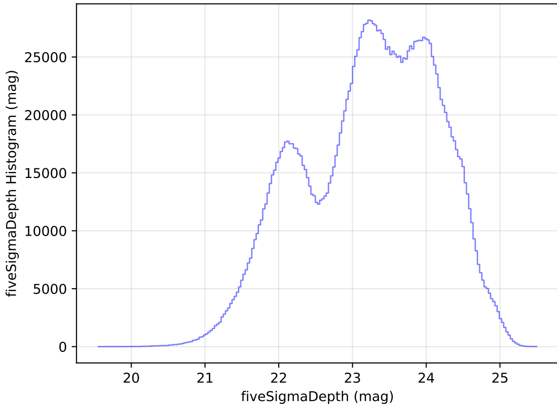
extra_ss_neo7_v3.4_10yrs All sky all bands: fiveSigmaDepth Histogram
