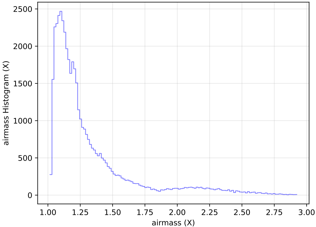
extra_ss_neo7_v3.4_10yrs Yr 1 z band: airmass Histogram
