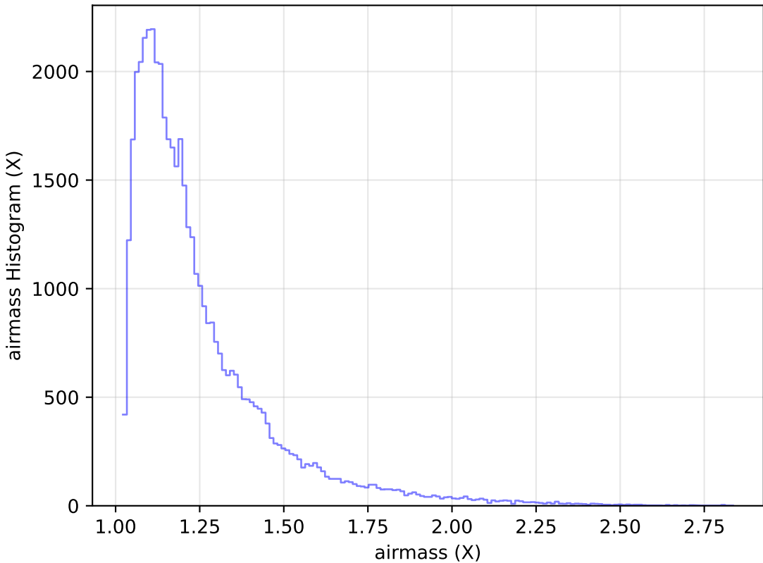
extra_ss_neo7_v3.4_10yrs Yr 1 y band: airmass Histogram
