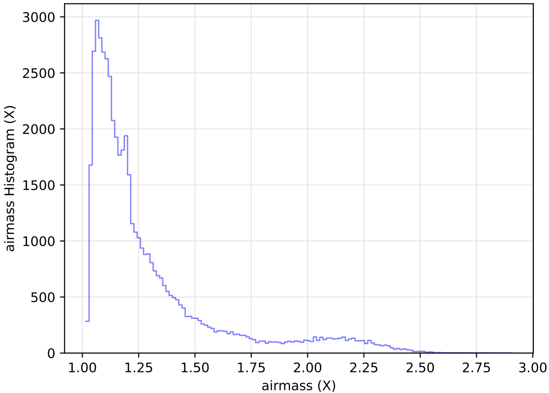
extra_ss_neo7_v3.4_10yrs Yr 1 r band: airmass Histogram
