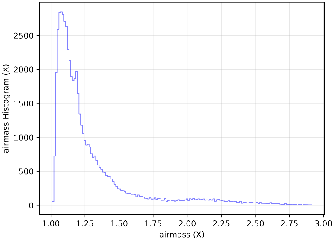
extra_ss_neo7_v3.4_10yrs Yr 1 i band: airmass Histogram
