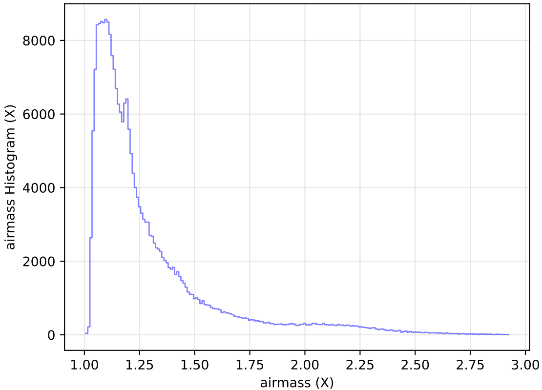
extra_ss_neo7_v3.4_10yrs Yr 1 all bands: airmass Histogram
